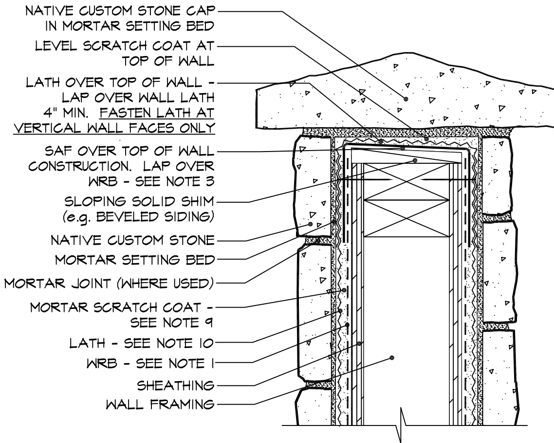
○ STONE WALL AND CAP SCALE: 3"=1'-0"
