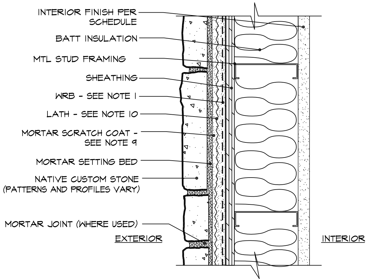
○ STONE OVER SHEATHING W/ MTL STUDS SCALE: N.T.S.
